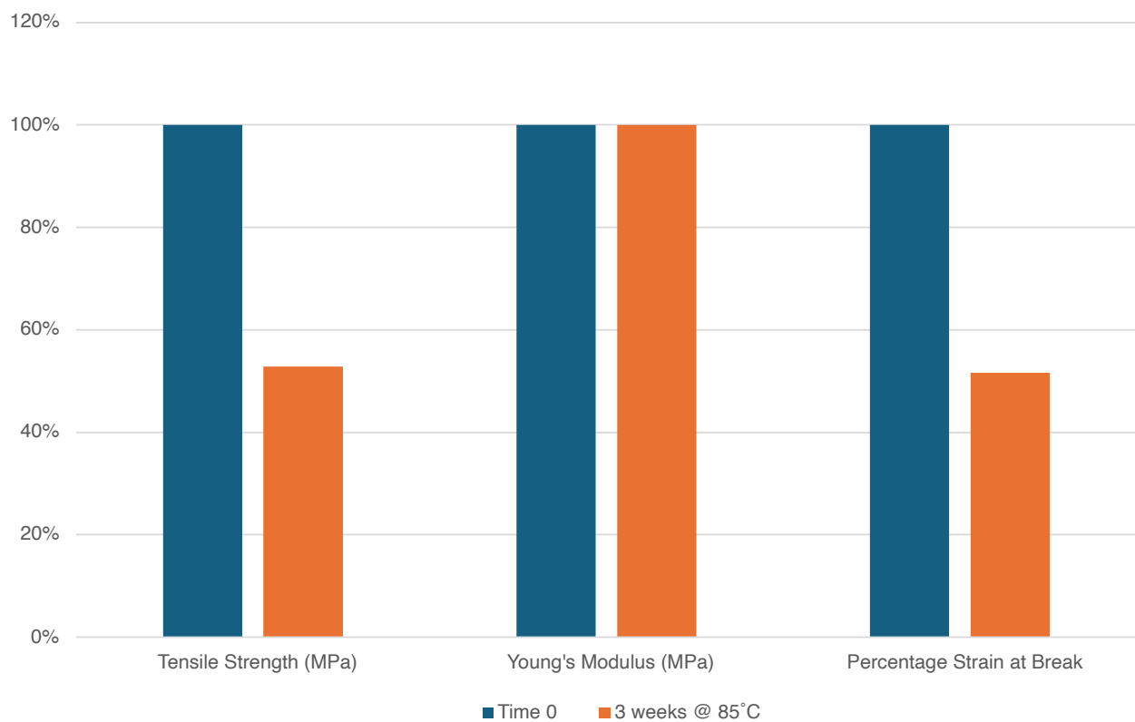
Mechanical properties after aging 3 weeks @ 85°C
