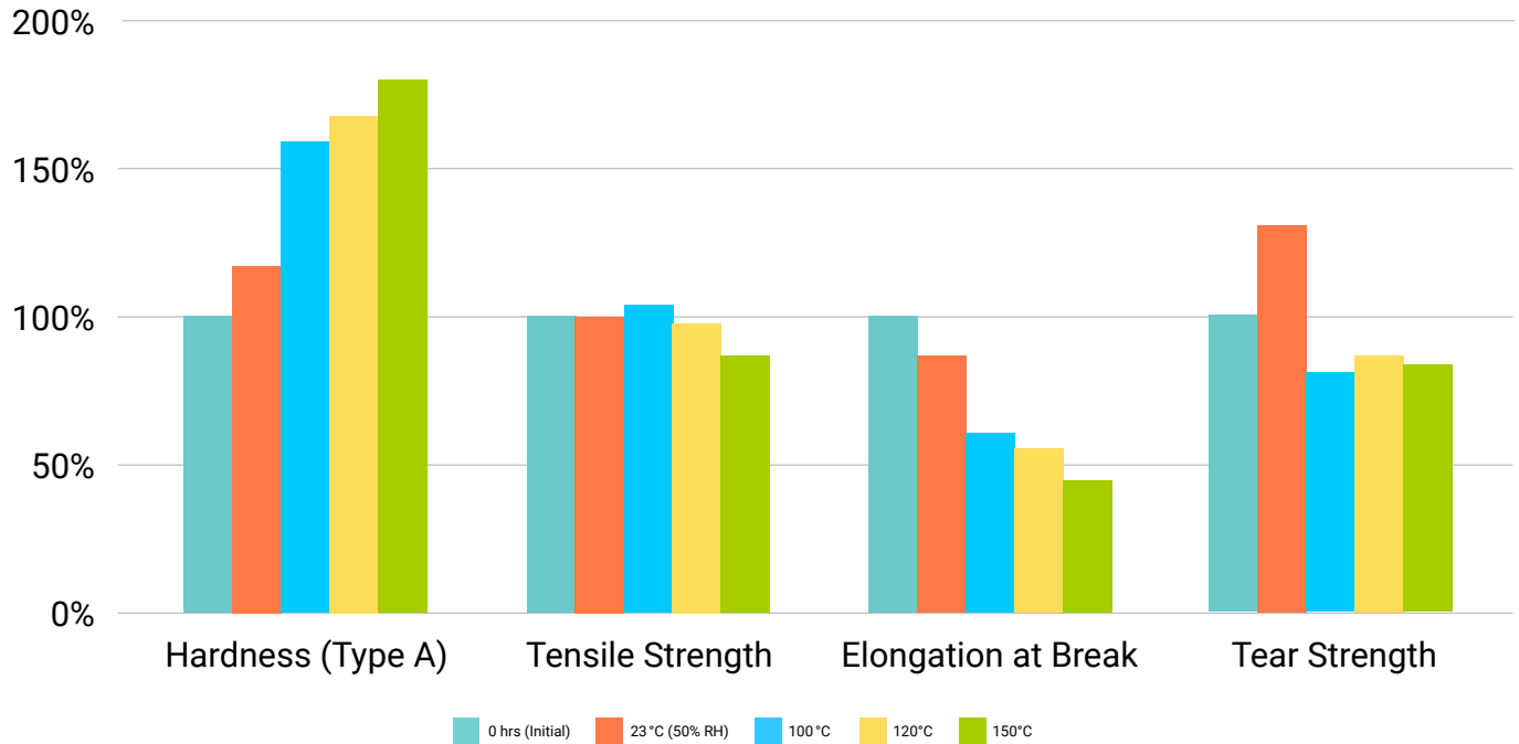
Mechanical properties after aging in different temperatures after 1,000 hrs
